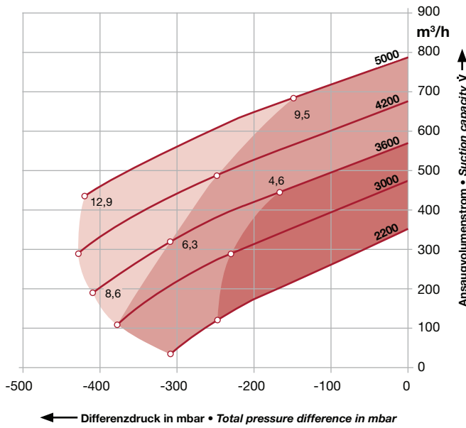
2BH2 0540 einstufig · single stage
