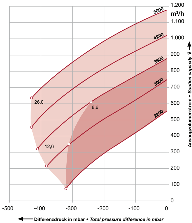
2BH2 0780 einstufig · single stage
