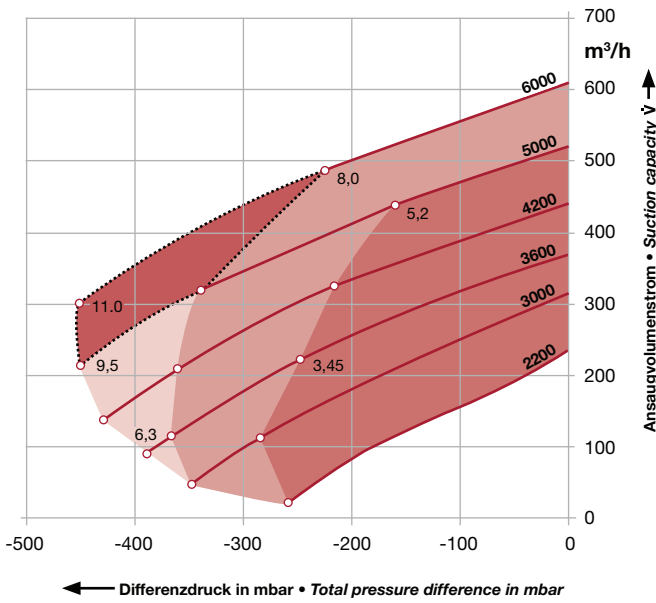
2BH2 0360 einstufig · single stage
